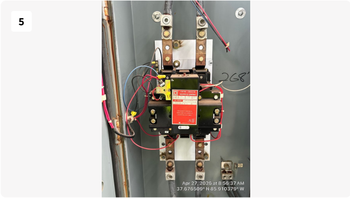
400Amp Contactor
