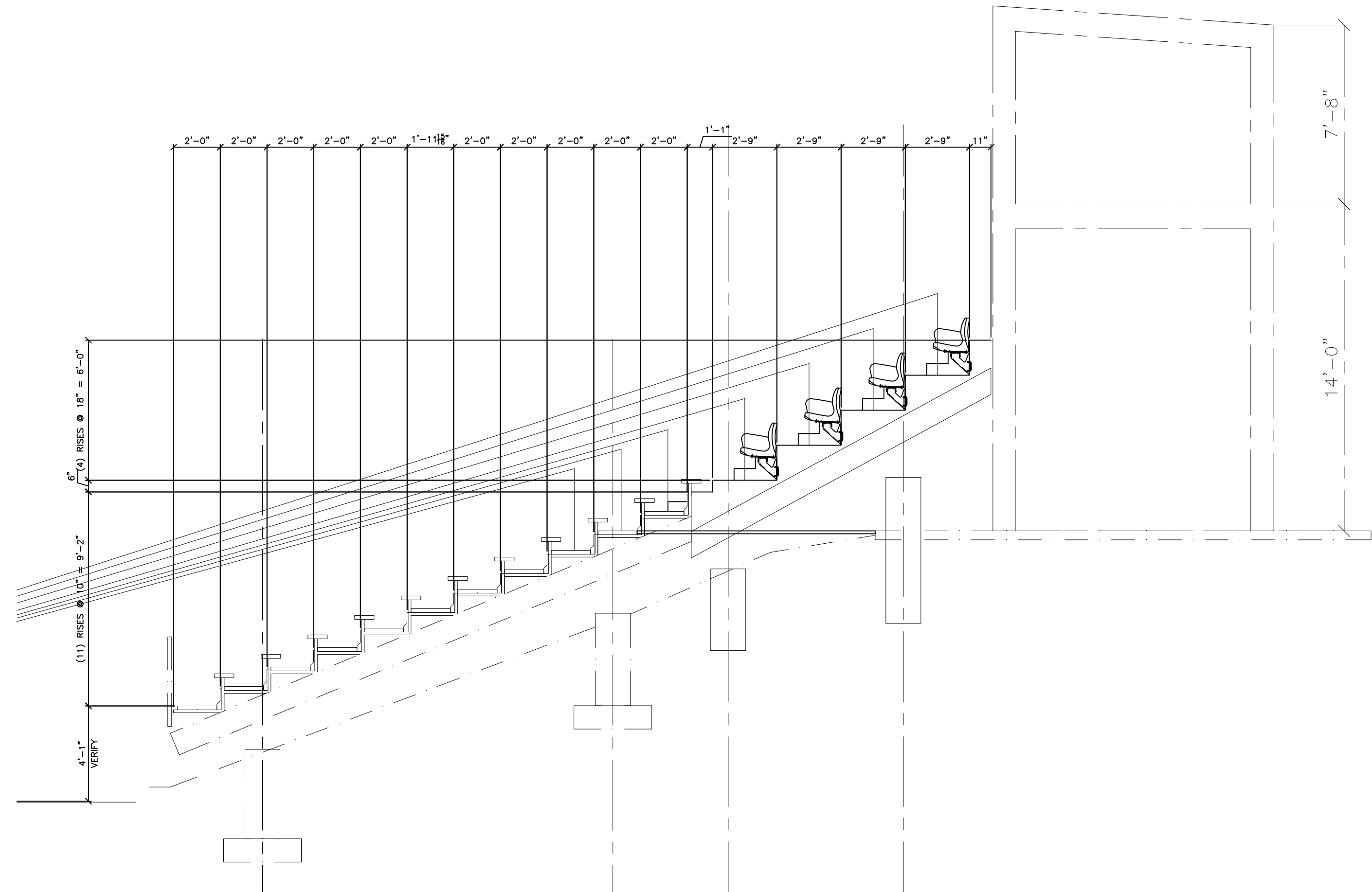
2 SECTION THRU CENTER GRANDSTAND AT PRESSBOX SCALE: 1/4" = 1'-0"
