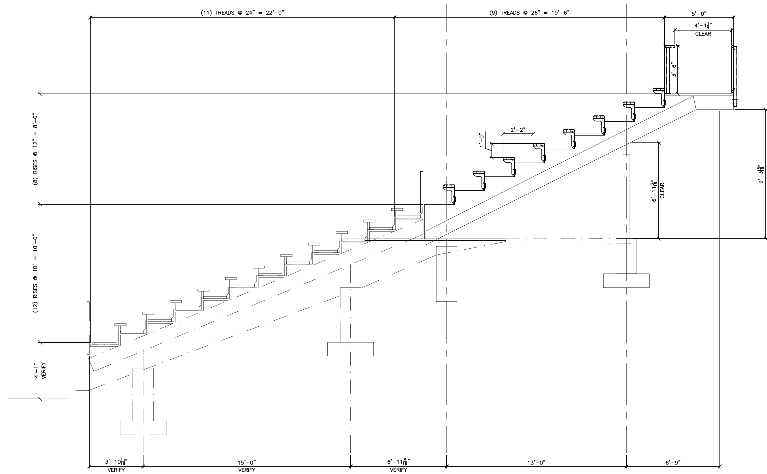
1 SECTION THRU WINGS 12" / 26" RISE/RUN SCALE: 1/4" = 1'-0"
