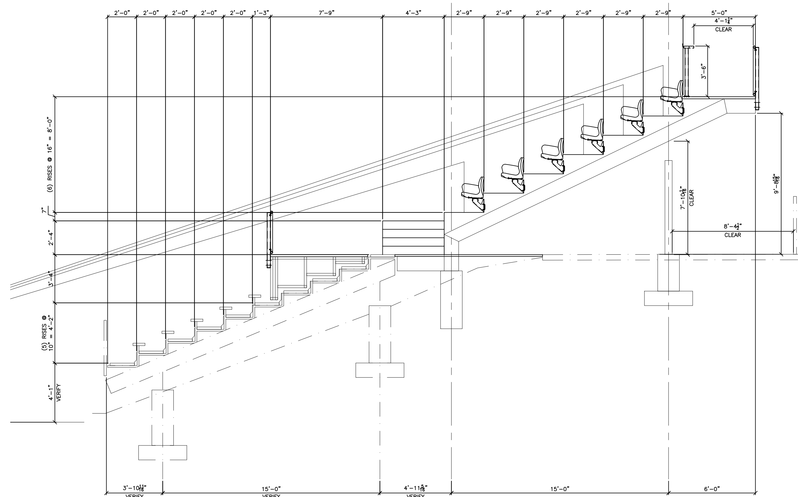
3 SECTION THRU WINGS 16" / 33" RISE/RUN SCALE: 1/4" = 1'-0"
