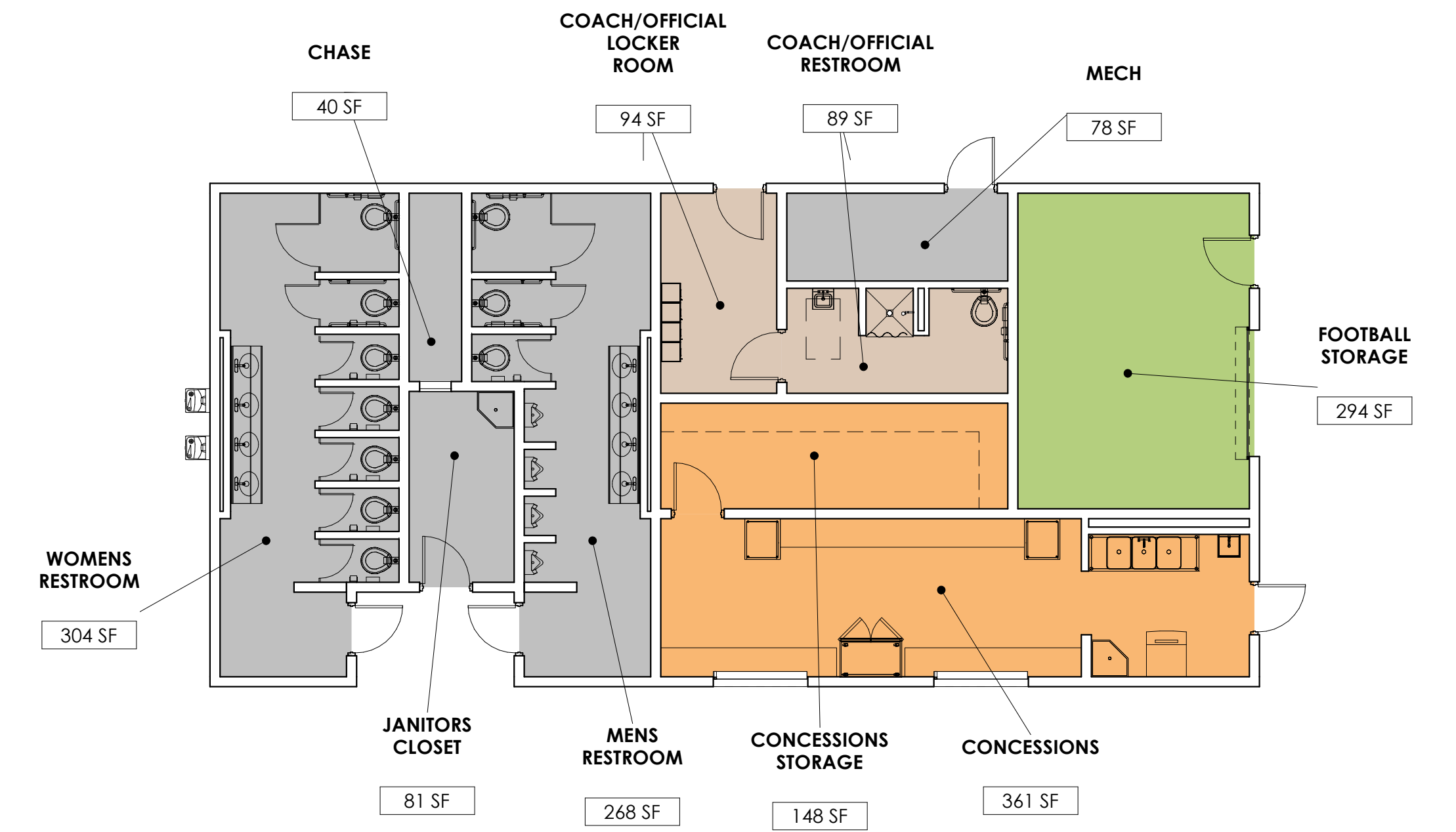
SCHEMATIC DESIGN FLOOR PLAN - CONCESSIONS/RESTROOM: OVERALL BUILDING FOOTPRINT - 2,130 SF
