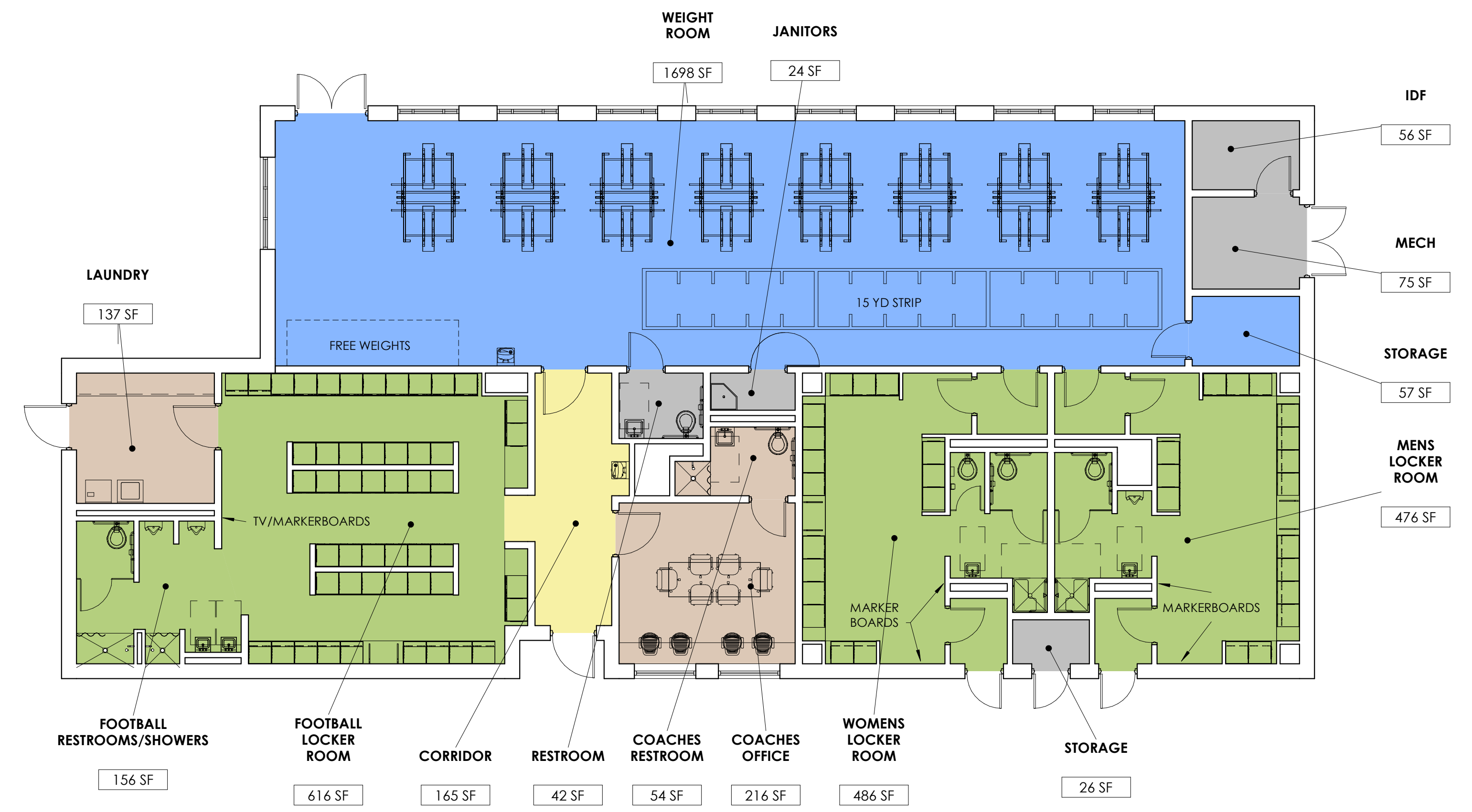
SCHEMATIC DESIGN FLOOR PLAN - LOCKER/WEIGHT ROOM: OVERALL BUILDING FOOTPRINT - 5,083 SF
