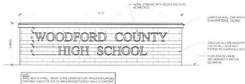
MONUMENT SIGN ELEVATION SCALE: 1/2" = 1'-0"
