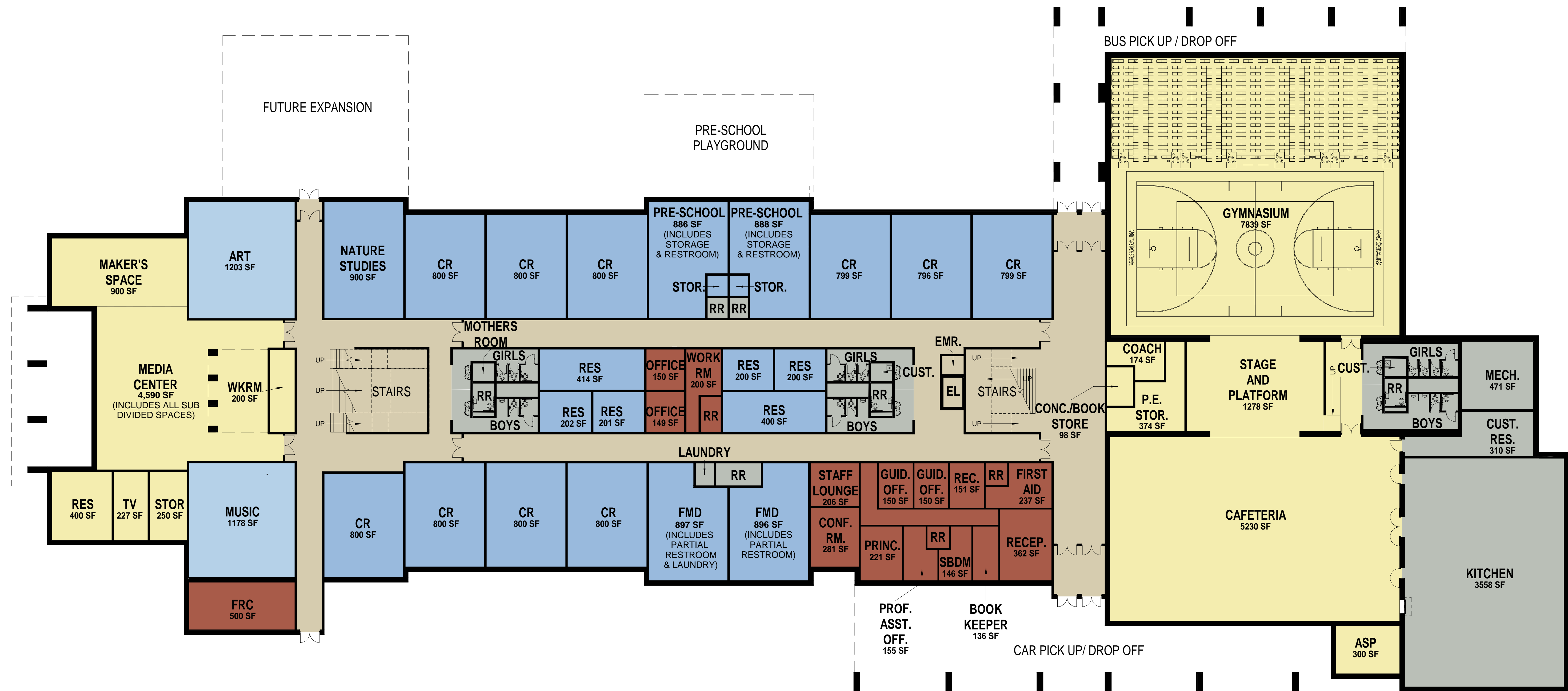
1 FIRST FLOOR PLAN 1/16" = 1'-0"
