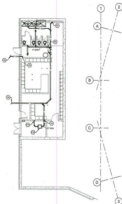
1 SOHS CONCESSIONS LOWER LEVEL - UNDERSLAB PLUMBING SCALE: 1/8" = 1'-0"
