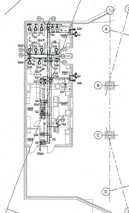
3 SOHS CONCESSIONS LEVEL 1 - PLUMBING
