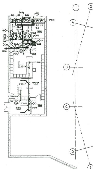
2 SOHS CONCESSIONS LOWER LEVEL - PLUMBING
