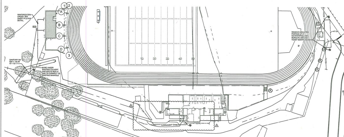
4 PLUMBING SITE PLAN - SOUTH OLDHAM HIGH SCHOOL SCALE: 1" = 30'-0"
