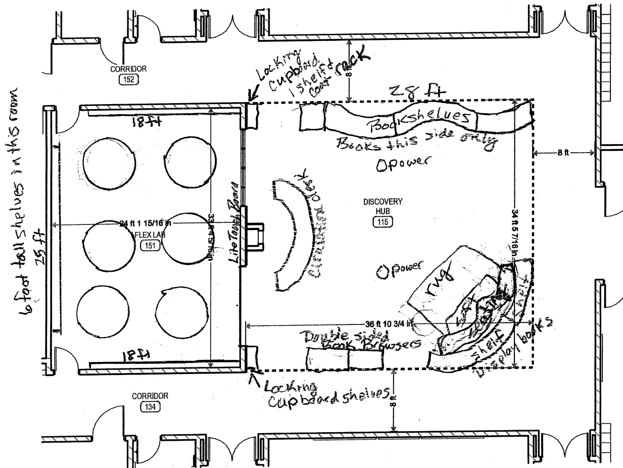
1 ENLARGED DISCOVERY HUB 1/8" = 1'-0"
