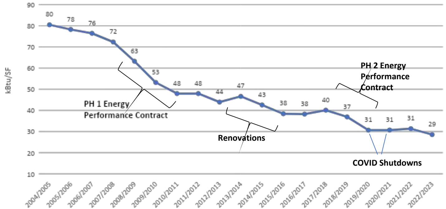
District Energy Journey – Energy Use Intensity (EUI) Total Energy per Square Ft
