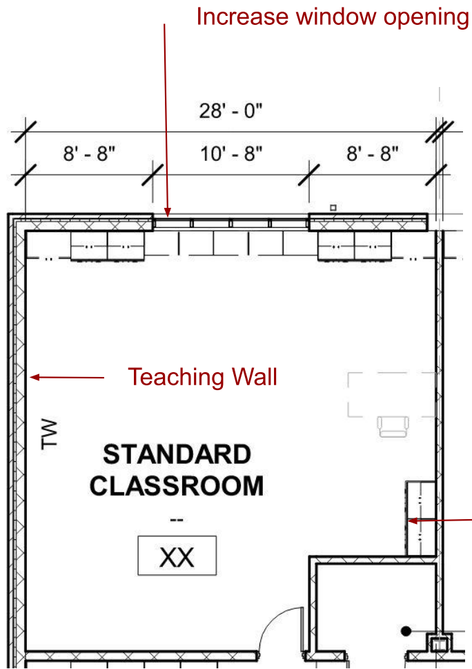
Standard Classroom Layout
