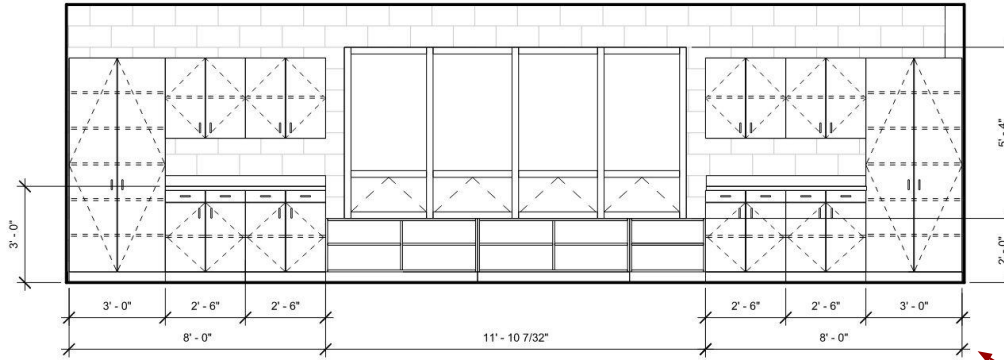
① CLSRM STORAGE ELEVATION- TYP. 3/8" = 1'-0"
