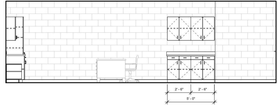
② CLSRM TEACHER DESK ELEVATION- TYP. 3/8" = 1'-0"
