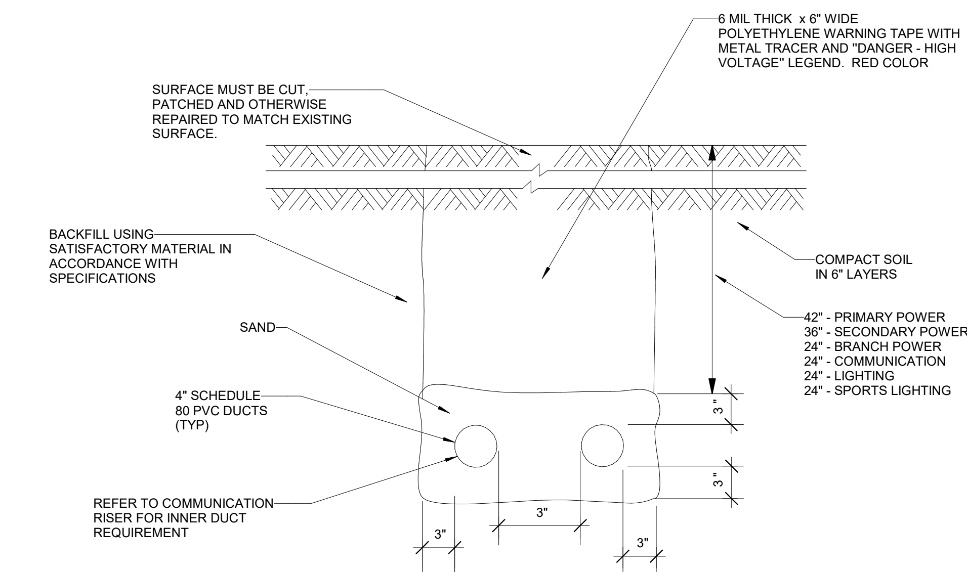
1 DUCTBANK DETAIL
