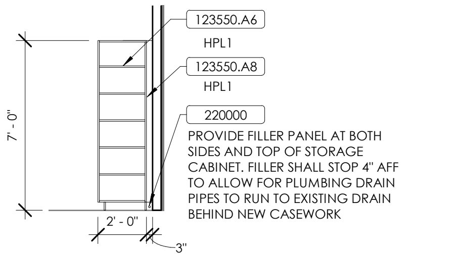
TALL CABINET SECTION 1/4" = 1'-0"
