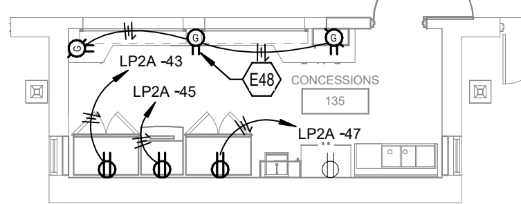
ENLARGED CONCESSIONS 135 POWER/SYSTEMS PLAN SCALE: 1/8" = 1'-0"
