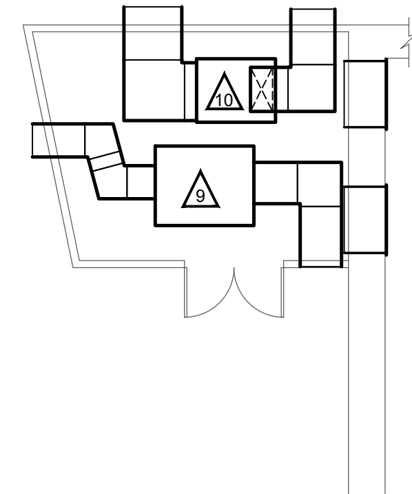
PROJECT NORTH SCALE: 1/8" = 1'-0" UPPER LEVEL LOFT/WORKROOM PLAN (ABOVE MEDIA CENTER)
