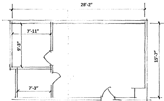
Partial floor Plan of Tech Building; Room #T-123
