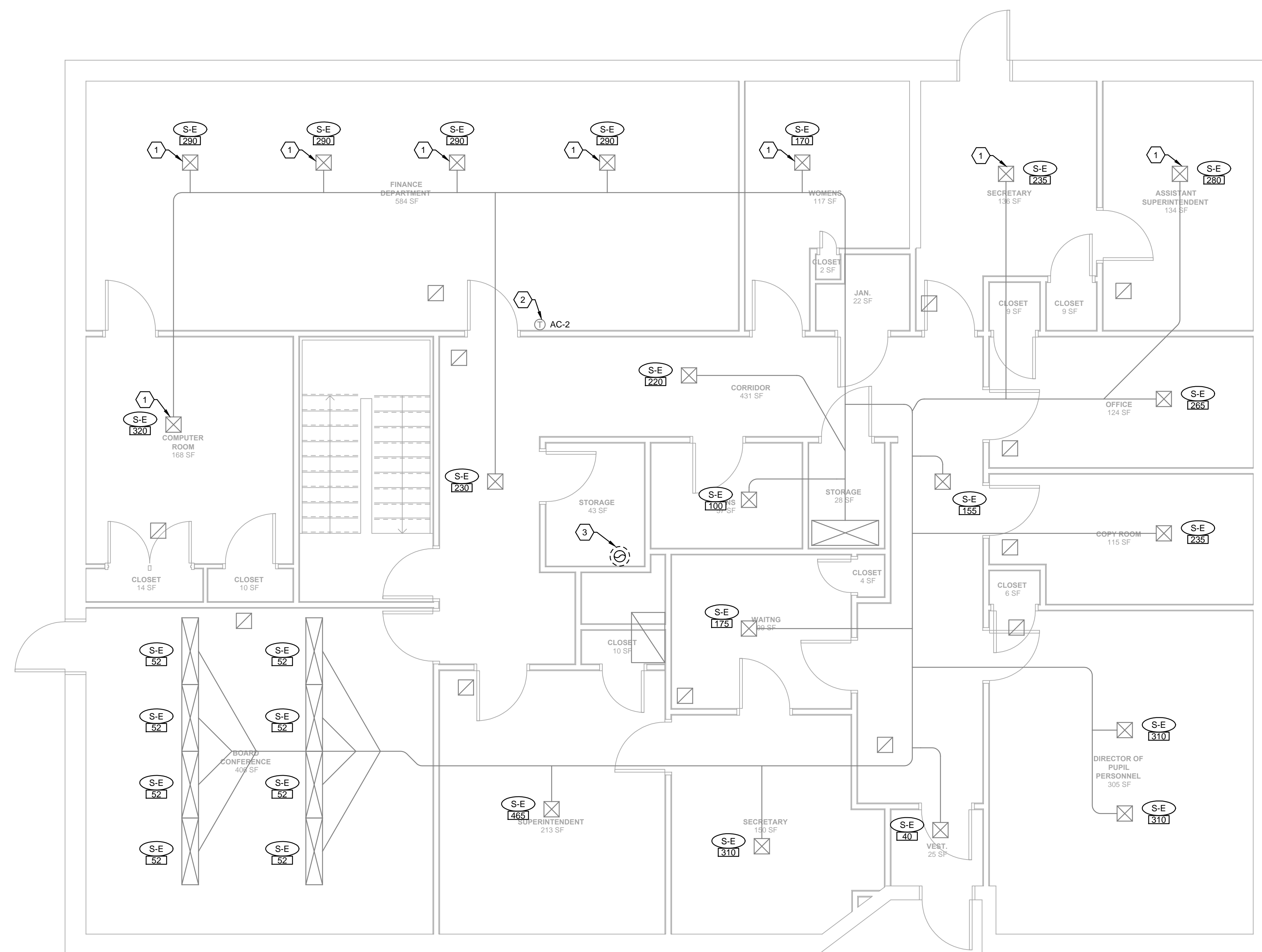
HVAC FIRST FLOOR PLAN - NEW WORK SCALE: 1/4" = 1'-0"
