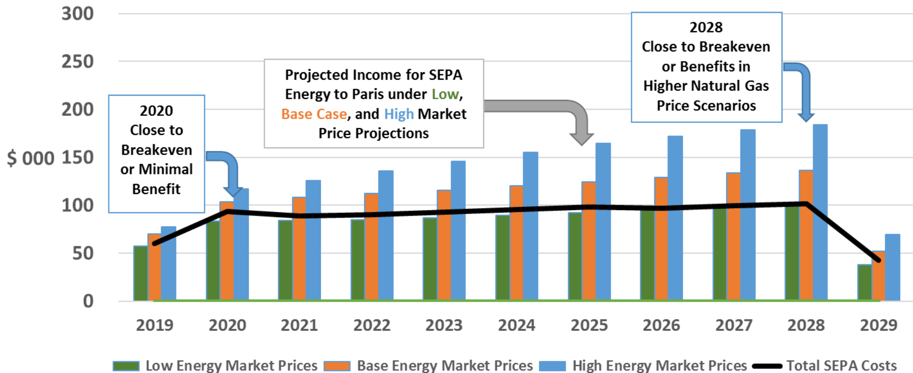
Options 2 or 3: Projected Income to Paris for SEPA Energy versus Projected Costs of SEPA - For Paris's 1.4 MW of SEPA Entitlement
