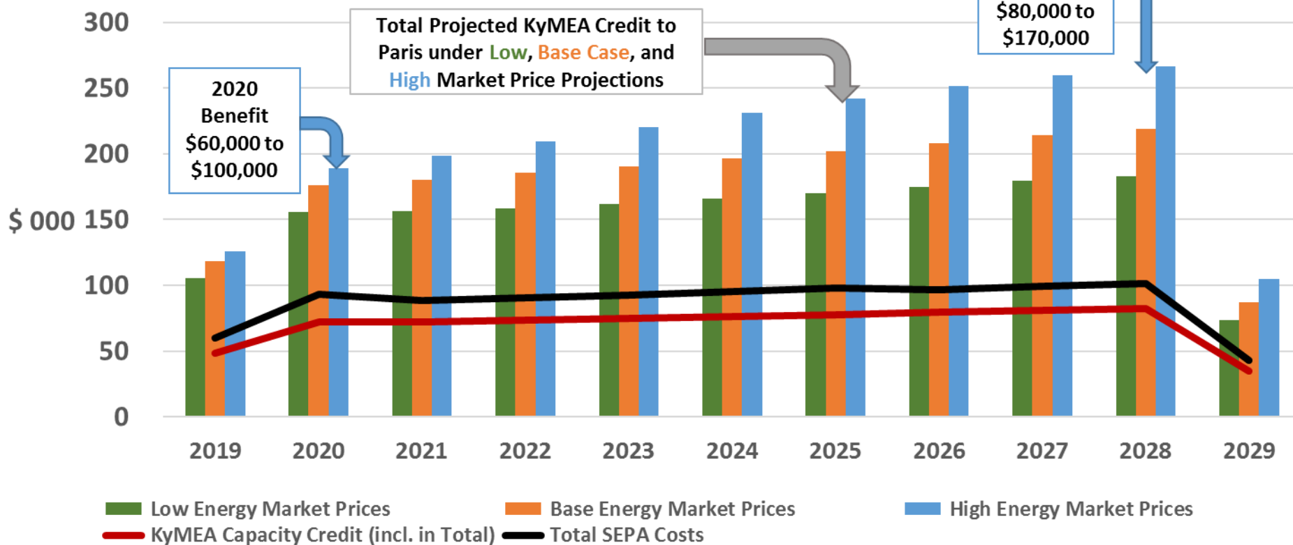
Option 1: Projected KyMEA Credits to Paris for SEPA Capacity and Energy versus Projected Costs of SEPA - For Paris's 1.4 MW of SEPA Entitlement
