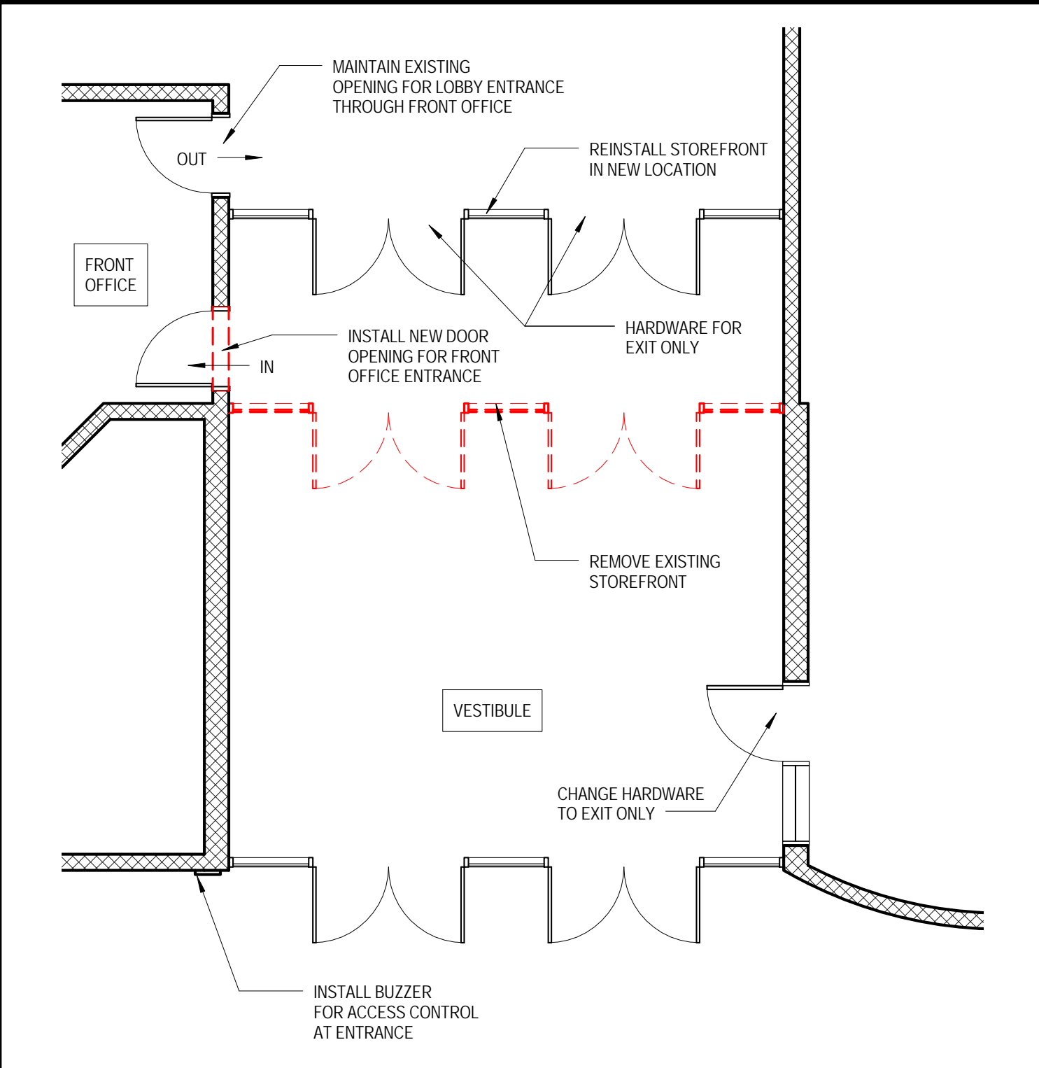
A VESTIBULE PLAN 3/16" = 1'-0"
