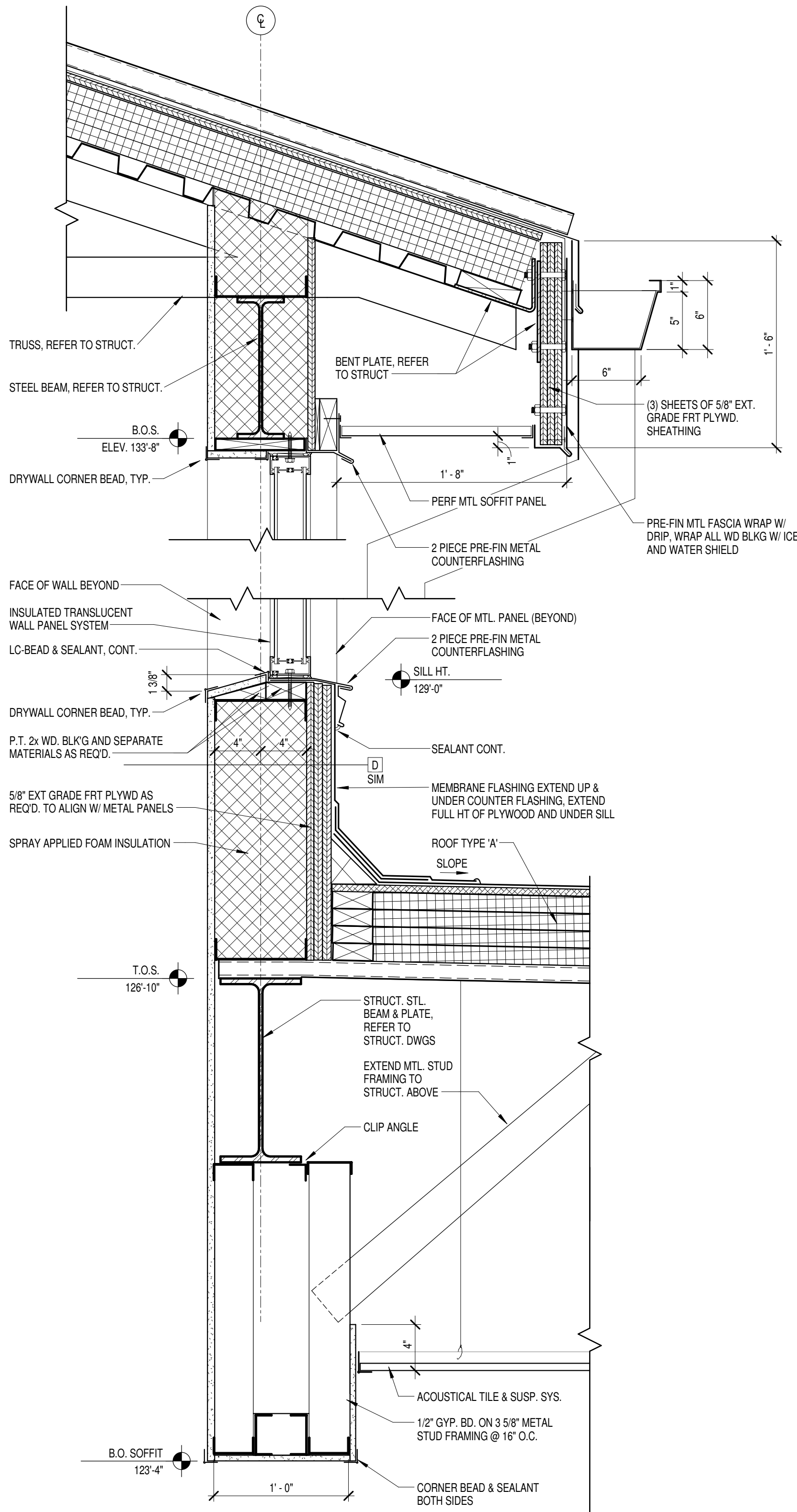
1 CLEARSTORY DETAIL 1 1/2" = 1'-0"
