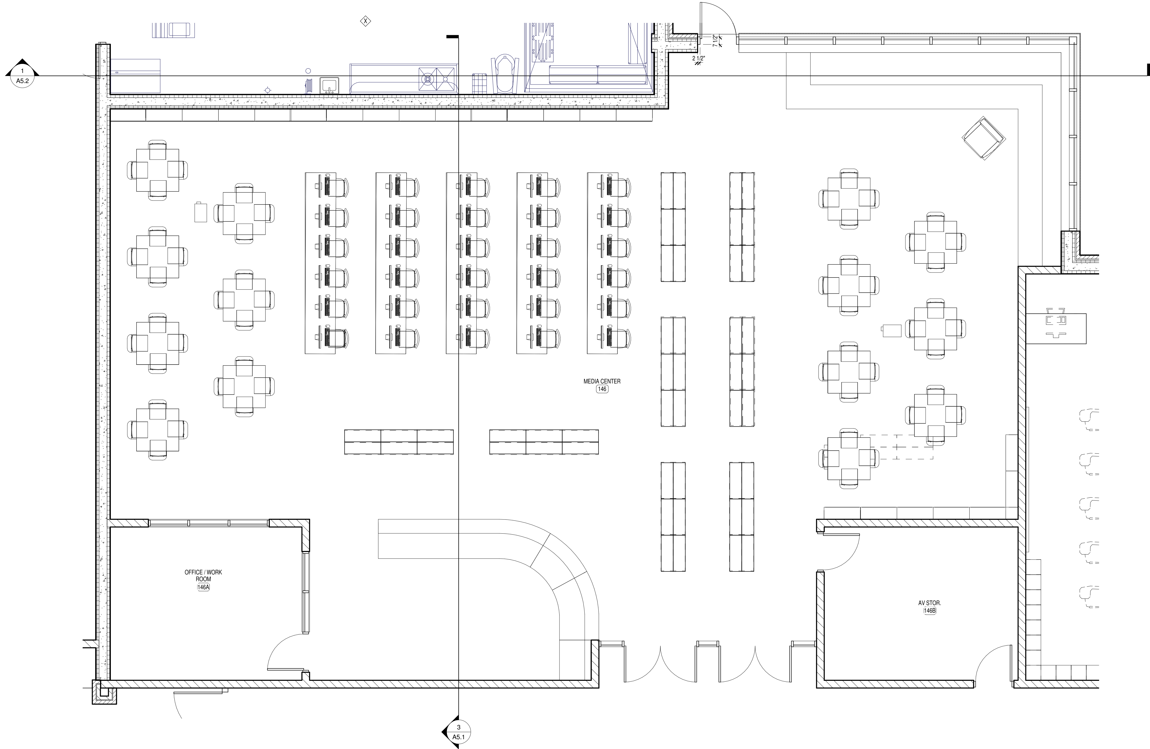
1 LEVEL 1 - 1/4" MEDIA CENTER 1/4" = 1'-0"
